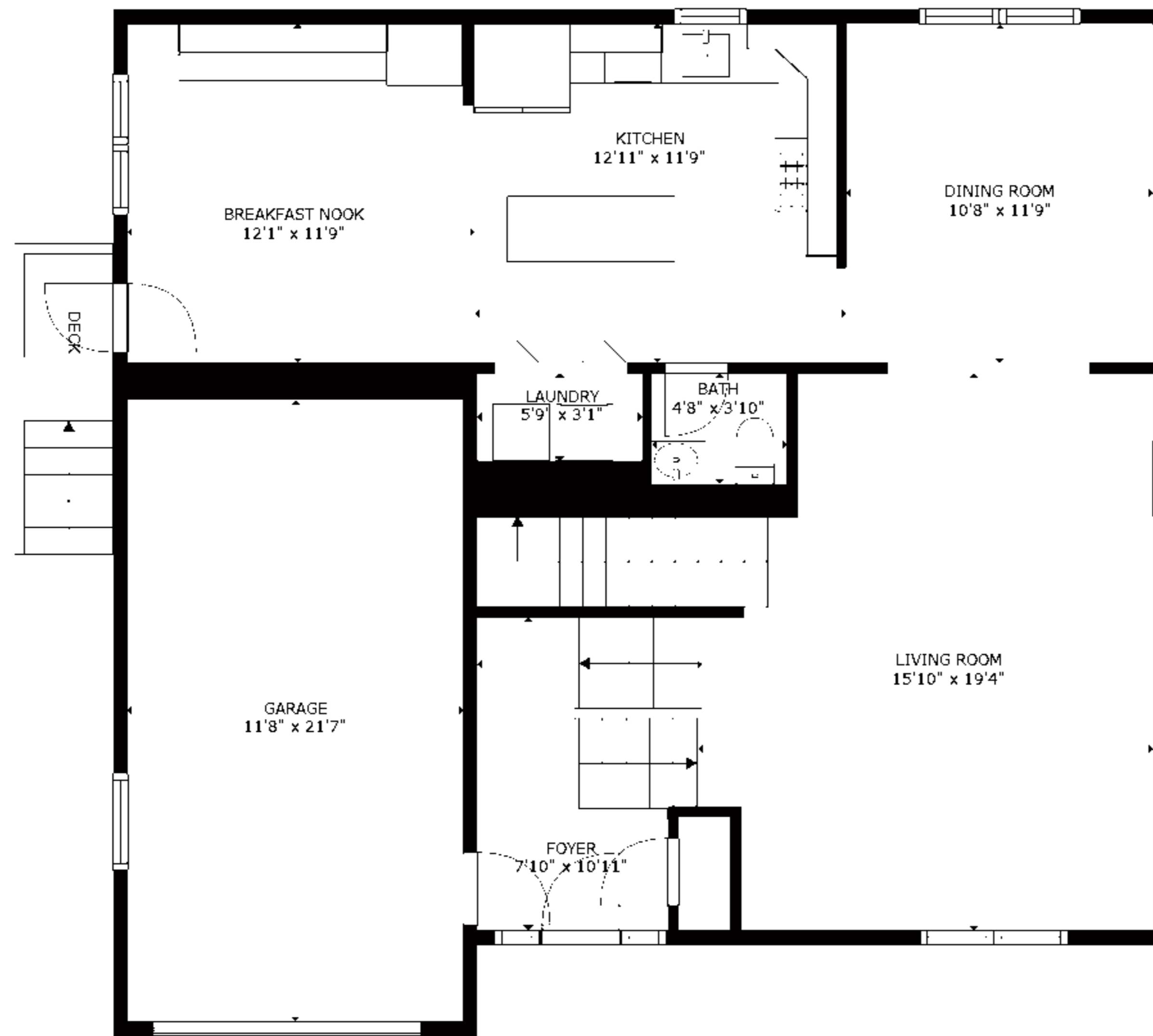
FLOOR 2
